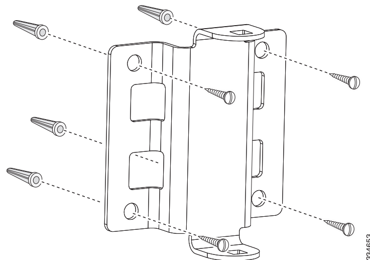
Figure 6 Wall Mounting
